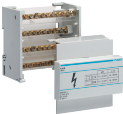
Brass busbar terminal 80A, 4pole
