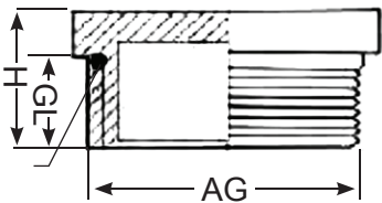
Sealing ring
